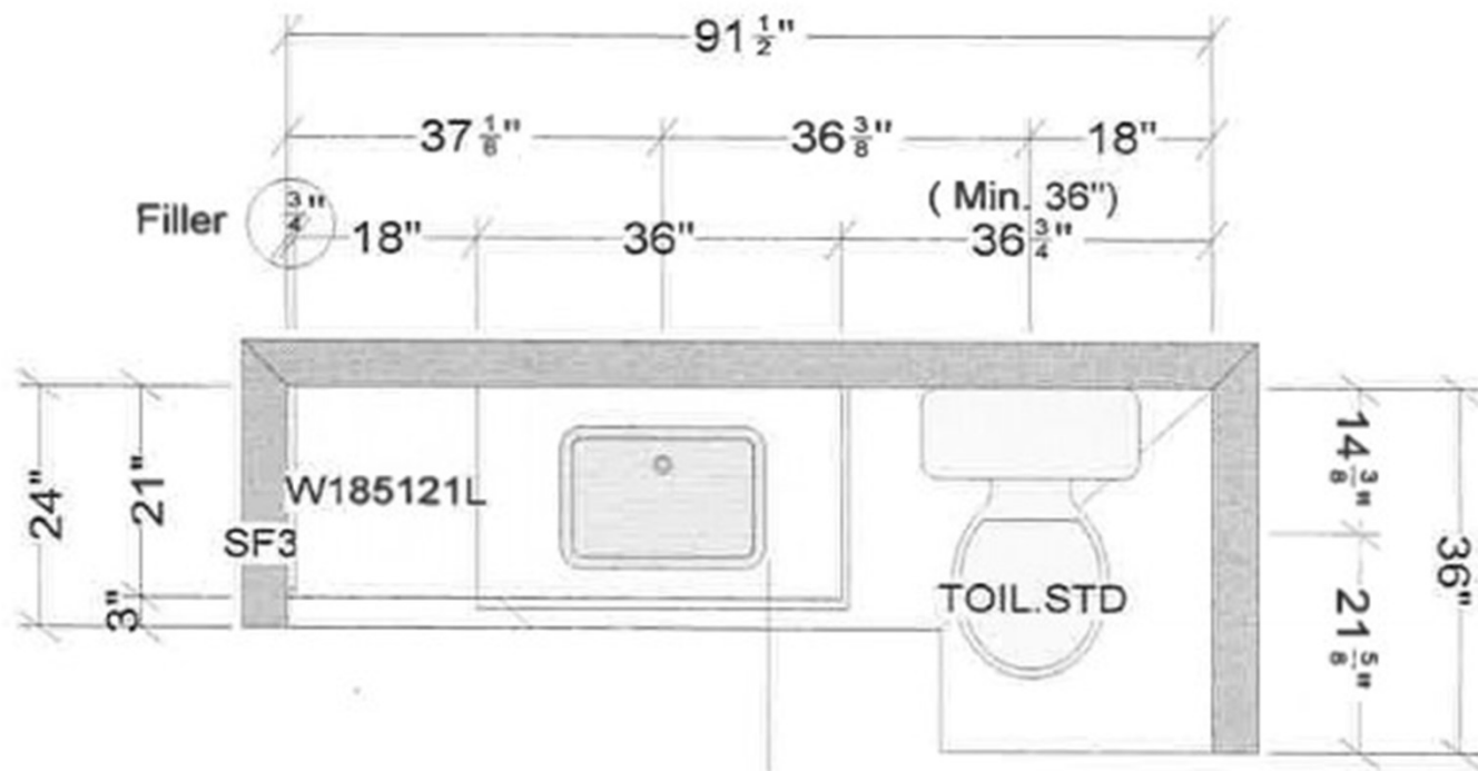
Removable Cabinet
