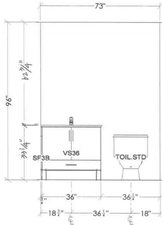
UNIT B3 PRIMARY BATH
