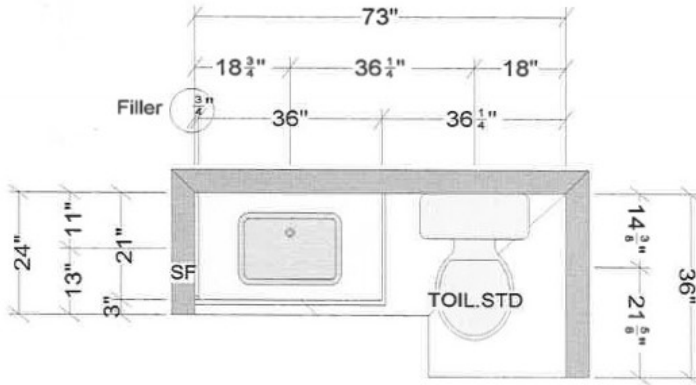
Unit B3 Primary Bath
