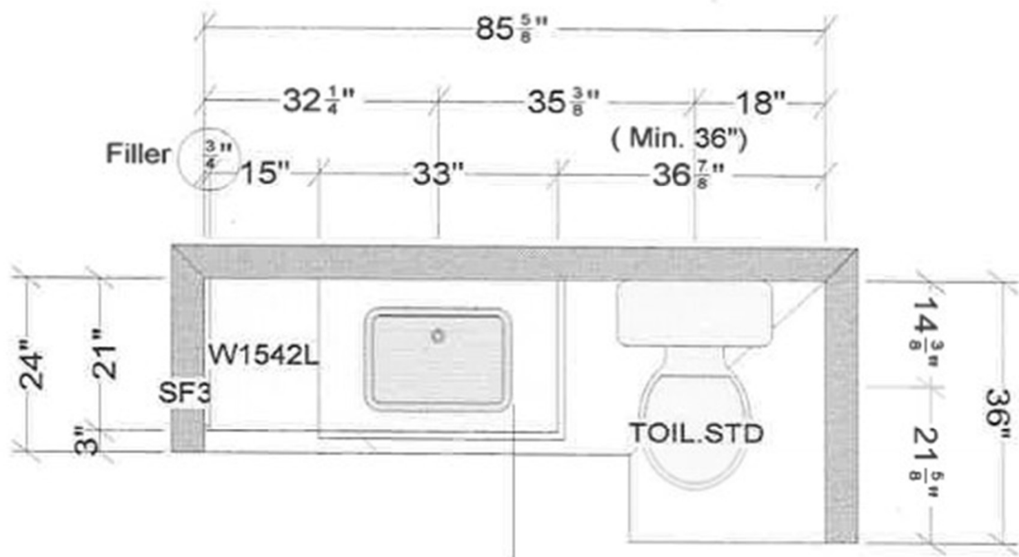
Removable Cabinet
